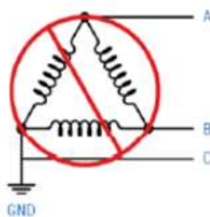
Corner Grounded
