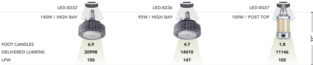
LIGHT DISTRIBUTION / FOOT CANDLE COMPARISON / DLC CEILING-MOUNTED HIGH BAY FIXTURES
