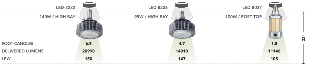
LIGHT DISTRIBUTION / FOOT CANDLE COMPARISON / DLC CEILING-MOUNTED HIGH BAY FIXTURES
