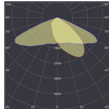
SL-AIO-70L AT 3000K
