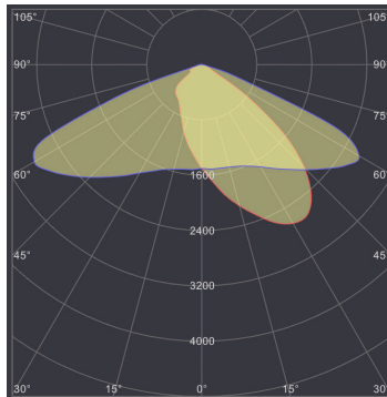
SL-AIO-70L AT 2700K
