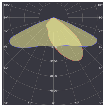
SL-AIO-70L AT 4000K
