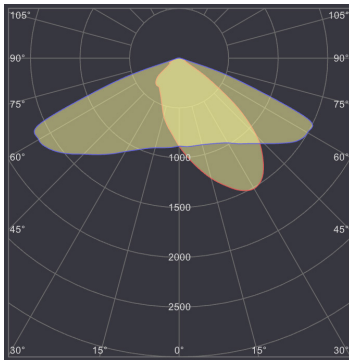
SL-AIO-40L AT 3000K
