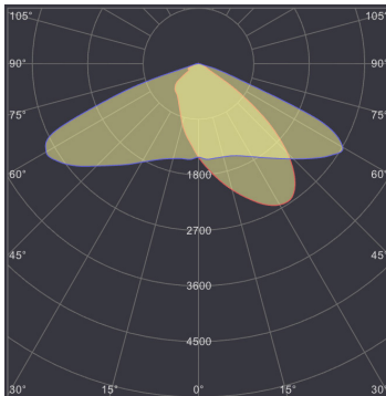
SL-AIO-70L AT 2200K
