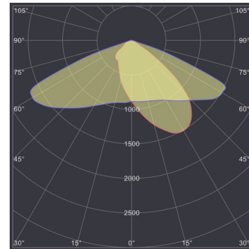
SL-AIO-40L AT 5000K
