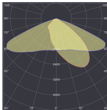
SL-AIO-70L AT 5000K
