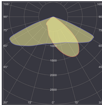
SL-AIO-40L AT 4000K
